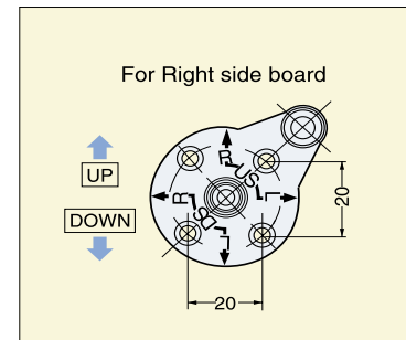
Mounting Plate SDS-A
